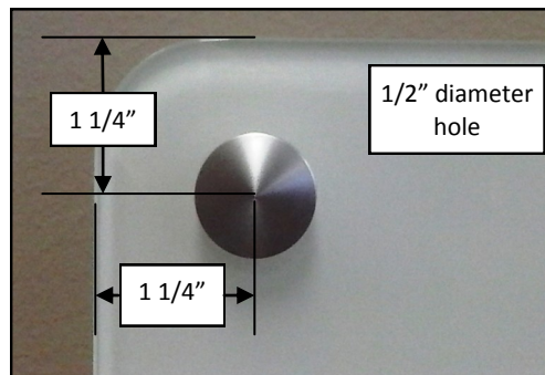
Corner profile
